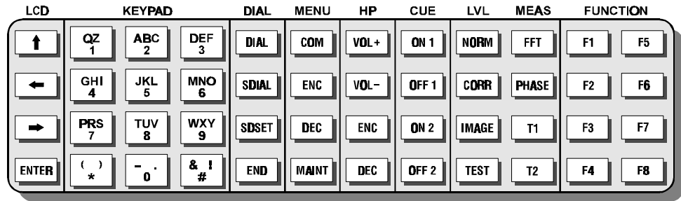
Figure 4-3 Model 230 keypad
