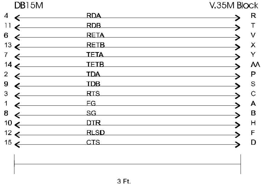
Cable C1300. DB15M To V.35 Block
