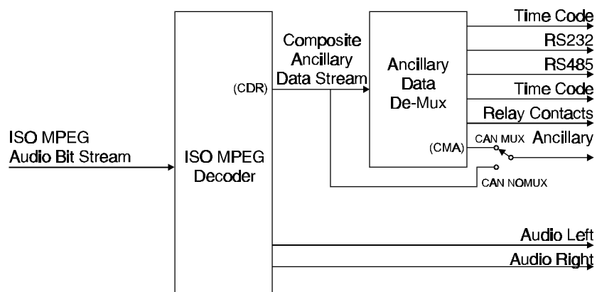
Figure 6-1 Async Data Mux/Demux Block Diagram
